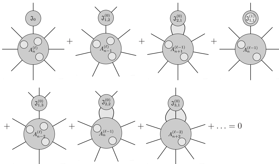
Figure 4. Expansion of quantum invariance of scattering amplitudes. Loops (light grey) can appear inside the amplitudes, inside the symmetry generator or in the connection of the two.
